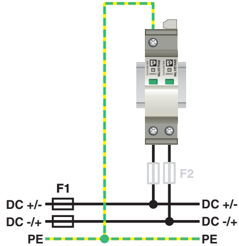
Product drawing
